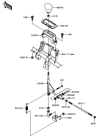
D-10 Control
